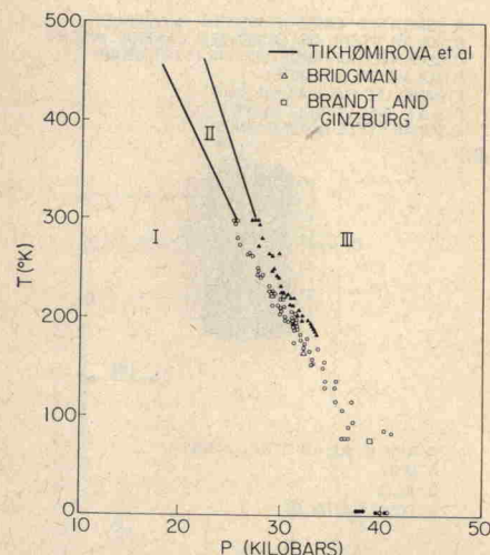
FIG. 5. The phase diagram of bismuth below room temperature as determined by the present author. The open circles represent the bismuth I-II or I-III phase boundaries. The closed triangles belong to the bismuth II-III phase boundary; however, the data points below about 225°K should not be used as an indication of the actual phase boundary because of the large uncertainty discussed in the text. The closed circles at 4.2°K represent one run in which the hysteresis loop was exceptionally small due to extrusion of some of the AgCl pressure-transmitting medium as described in the text. The open triangles refer to Bridgman's data (Ref. 1). The solid lines are straight lines drawn through the data of Tikhomirova et al. (Ref. 6). The open square is a point determined by Brandt and Ginzburg (Ref. 7).
